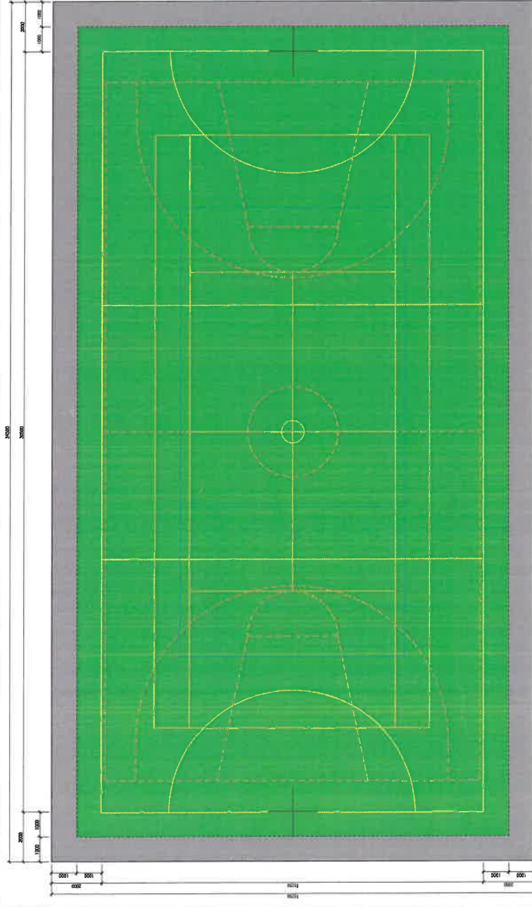
COMBO COURTS PLAN (1:50)
